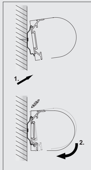
Wandmontage
