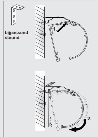
Wandmontage
